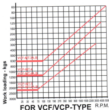
THE CHART FOR LOADING WEIGHT WITH R.P.M.
