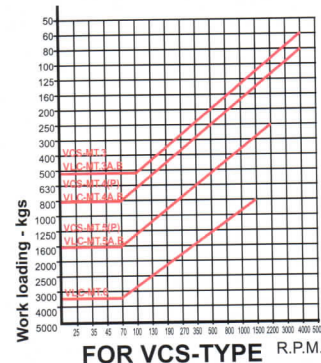
THE CHART FOR LOADING WEIGHT WITH R.P.M.
